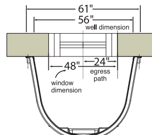
Top view with wall and window
